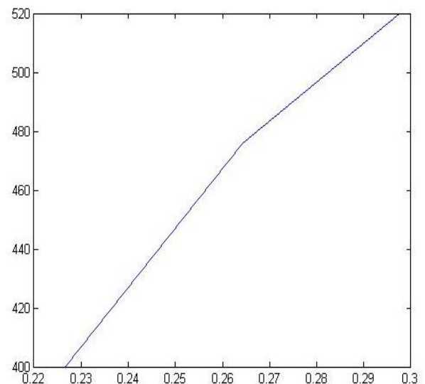
Fig. 6: Plot of Reactive Power Vs Load Current.
