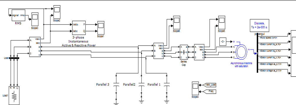
Fig. 1: Simulink Model of Long Shunt SEIG.
